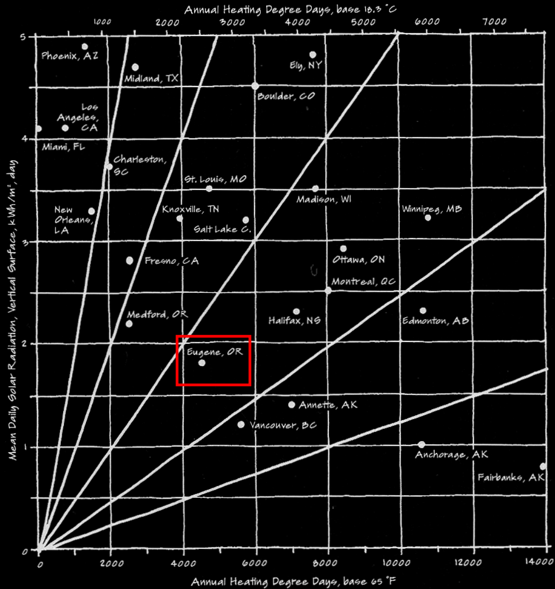
Heating Season Severity vs. January Radiation as an Indicator of Solar Heating Potential Diagonal lines show the ratio Degree Days/Radiation; Lower ratios indicate better solar heating potential.
