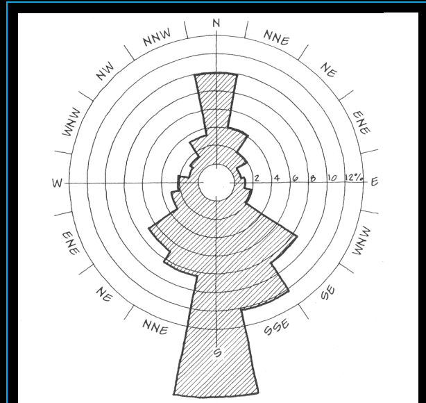
December Wind Rose, Eugene
